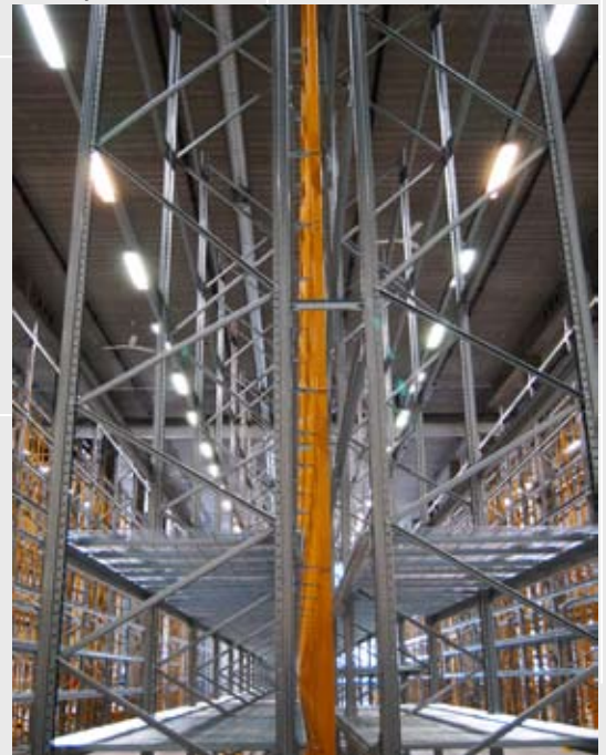
Pallet stoppers are efficient protection
